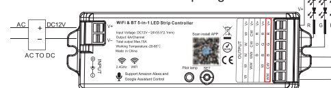
Connect to RGB+CCT LED strip diagram
